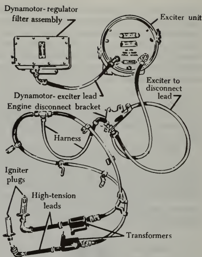
FIGURE 4-77. Typical electronic ignition system.
